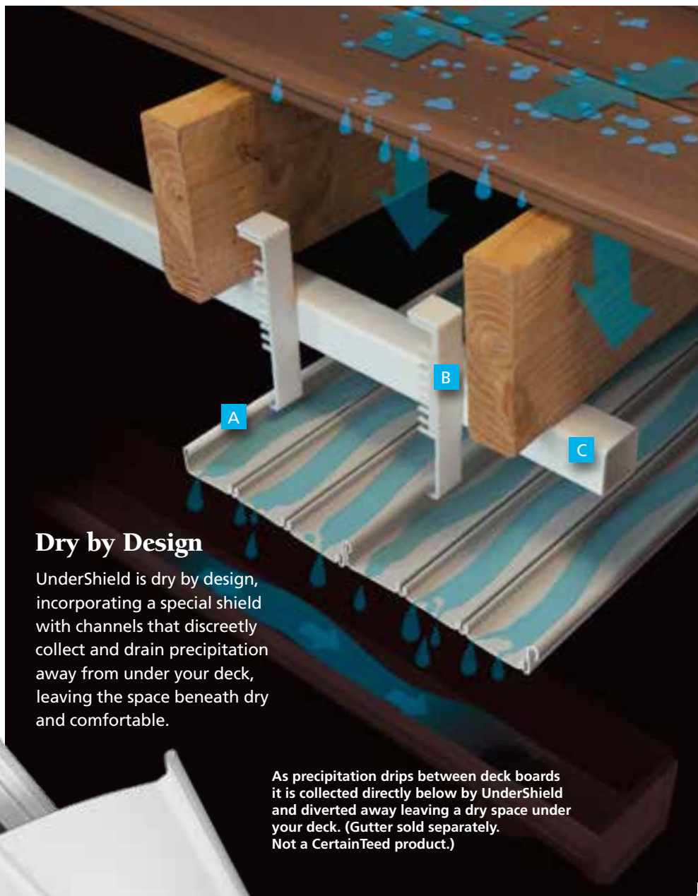
C Vinyl Grid System
