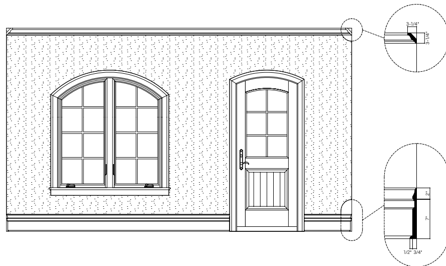
Quintessential Interior Room Trim
