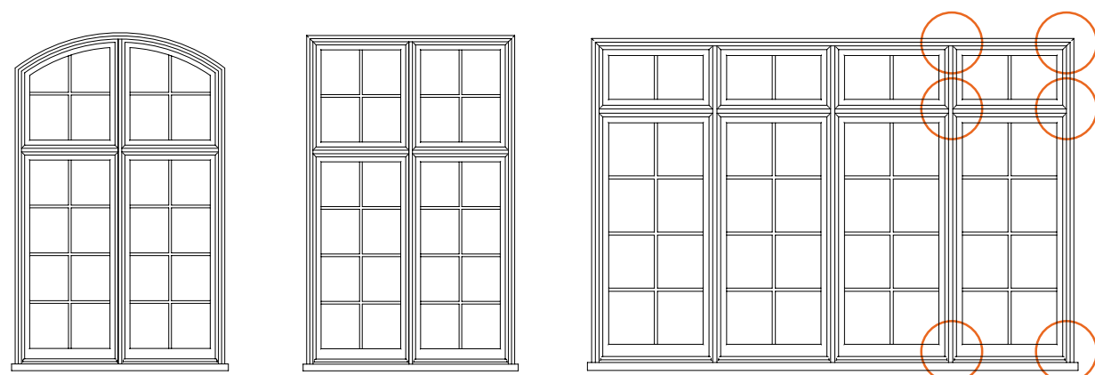
Two-wide casement window grouping with segmented arched transom windows
