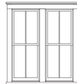
Alternate two-wide double-hung grouping. Jamb and mullion trim widths must match and be approximately 4 1/2" wide for central rosette to fit.
