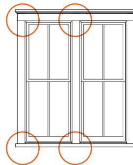
Two-wide double-hung grouping. +/- 5 1/2" mull is a very authentic size. Circled areas – See Typical Trim Conditions details on page 13.
