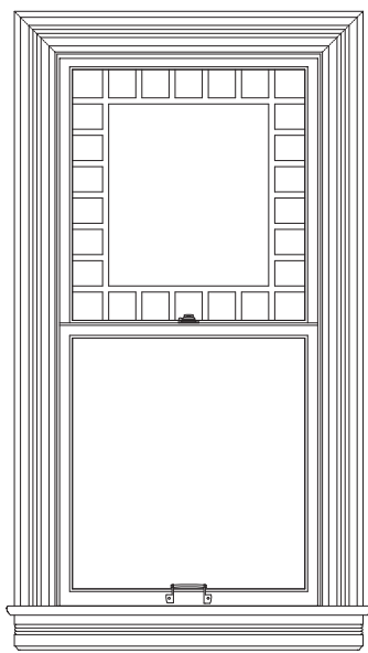
Triple-beaded casing with straight chamfer edge profile. Stool with elliptical bull edge. Apron cut from casing.
