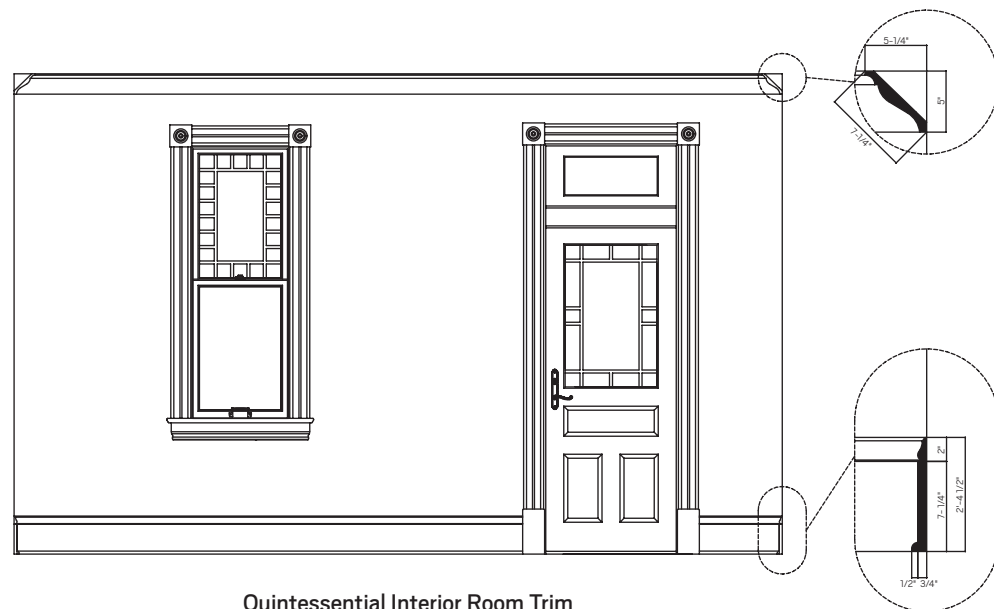
Quintessential Interior Room Trim
